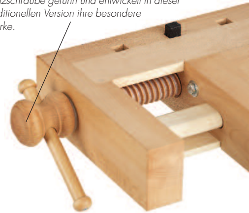
Adjustable shoulder vise with wooden screw.
